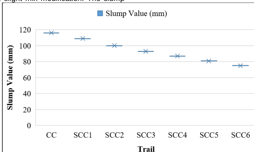
Figure 2. Slump Cone
