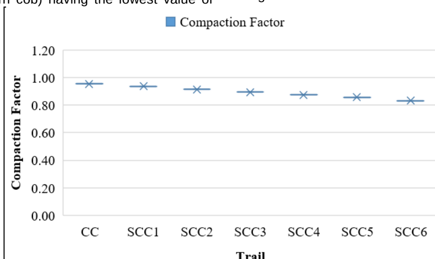
Figure 3. Compaction factor
